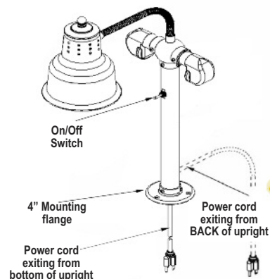
ESL-FM-600-BR Brass
